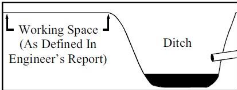
Figure 2. Cross-Section of an Open Ditch Municipal Drain.
