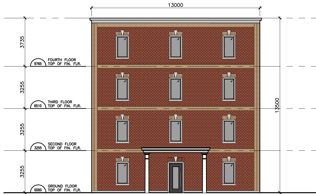
WEST ELEVATION
