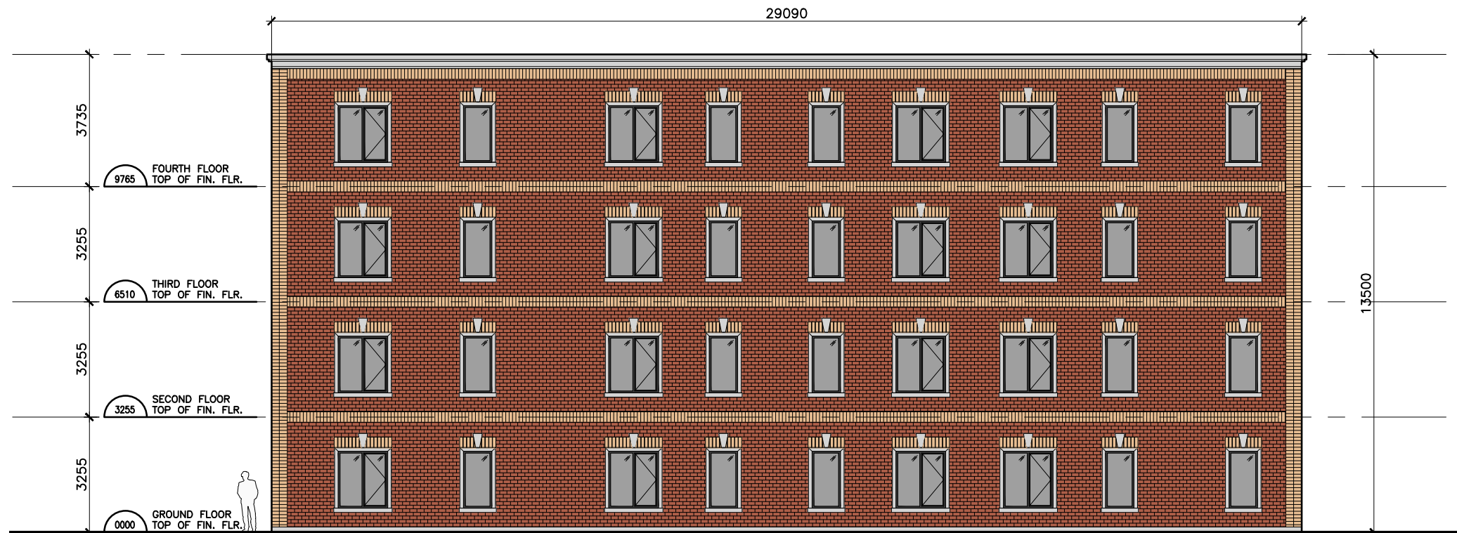
SOUTH ELEVATION
