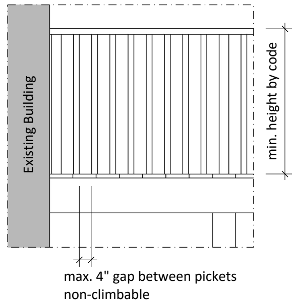
Guard Detail Scale: 1:25
